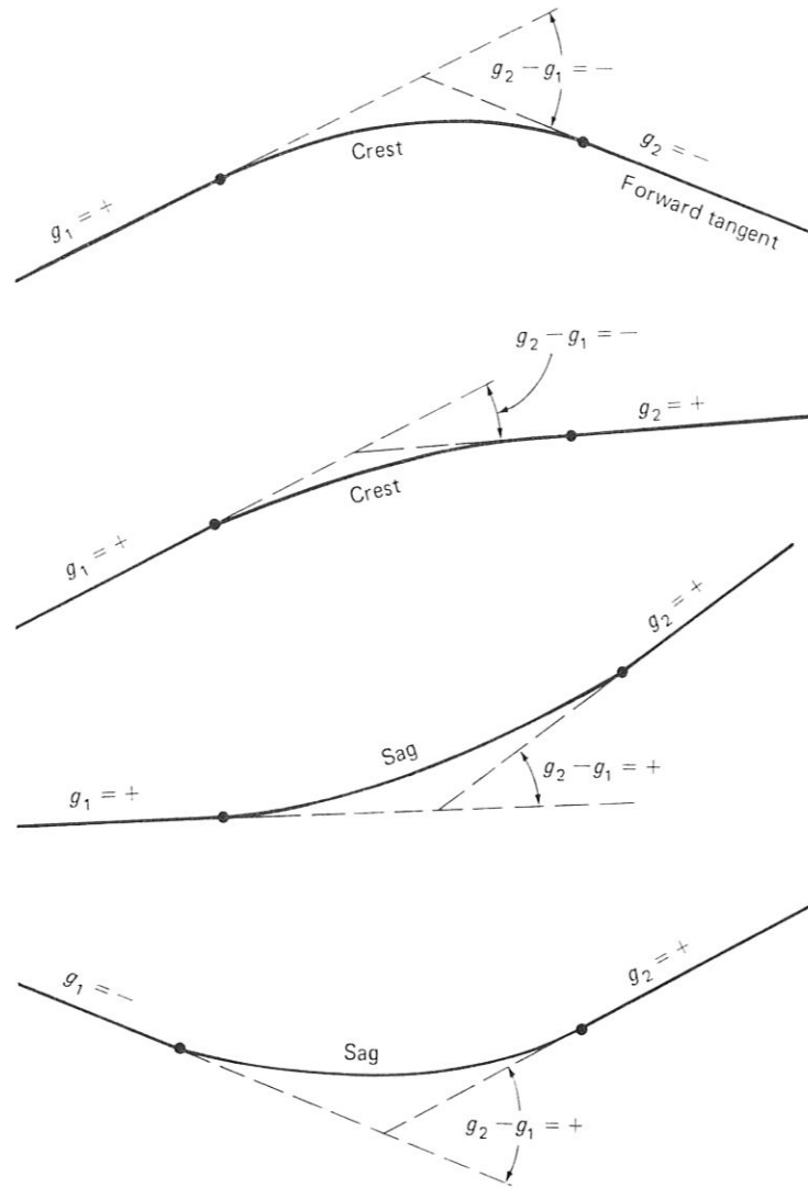
FIGURE 10-21 Vertical curves: crest and sag.
