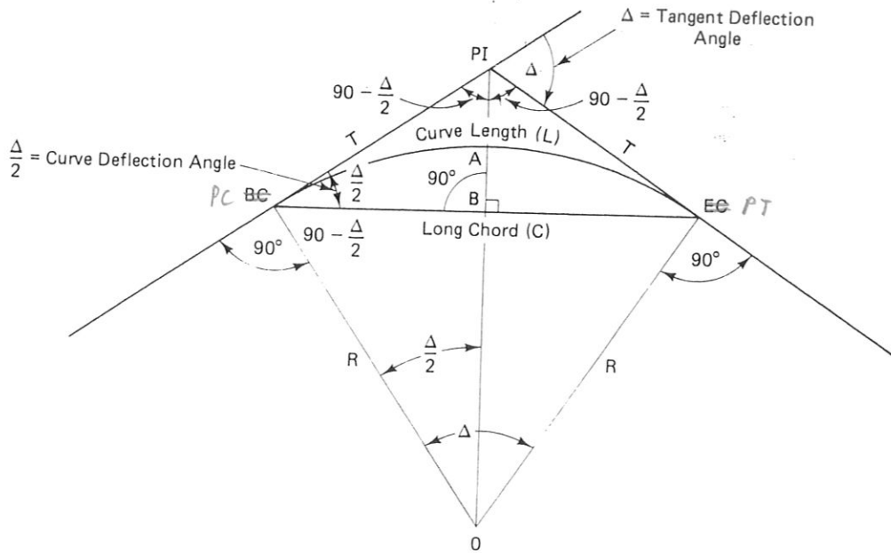
Figure 12-2 Geometry of the circle.
