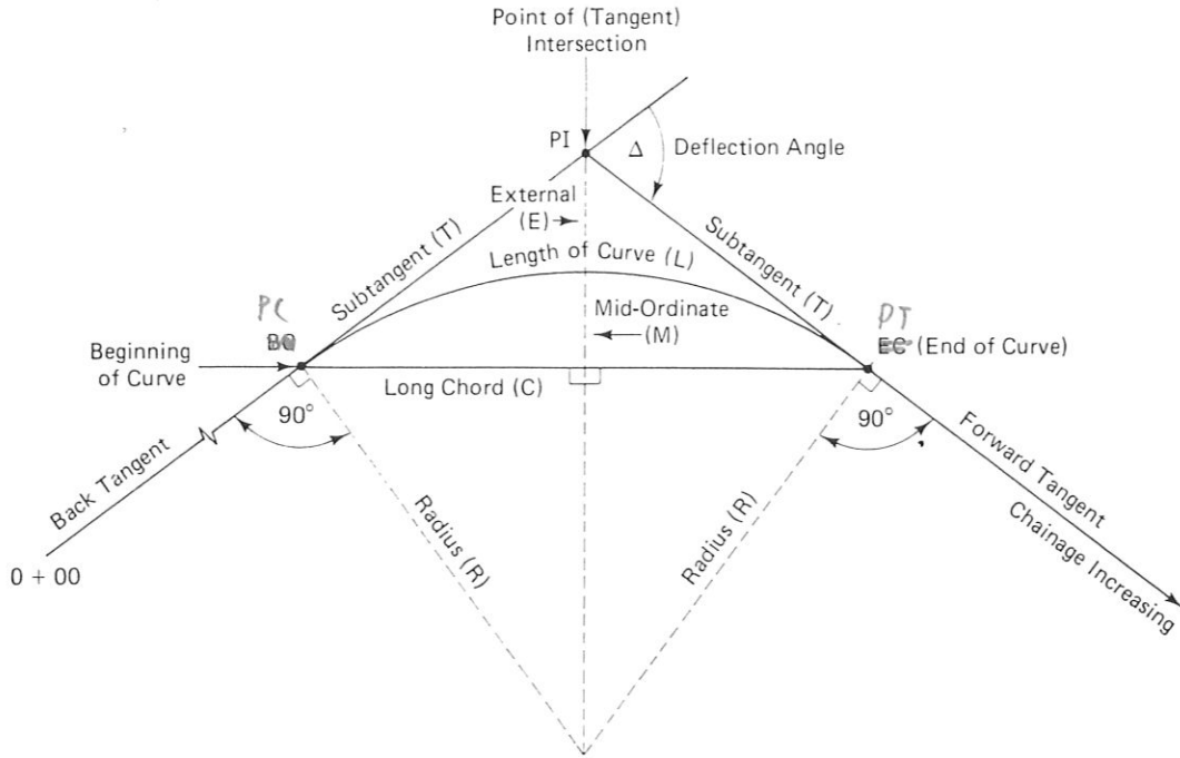
Figure 12-1 Circular curve terminology.
